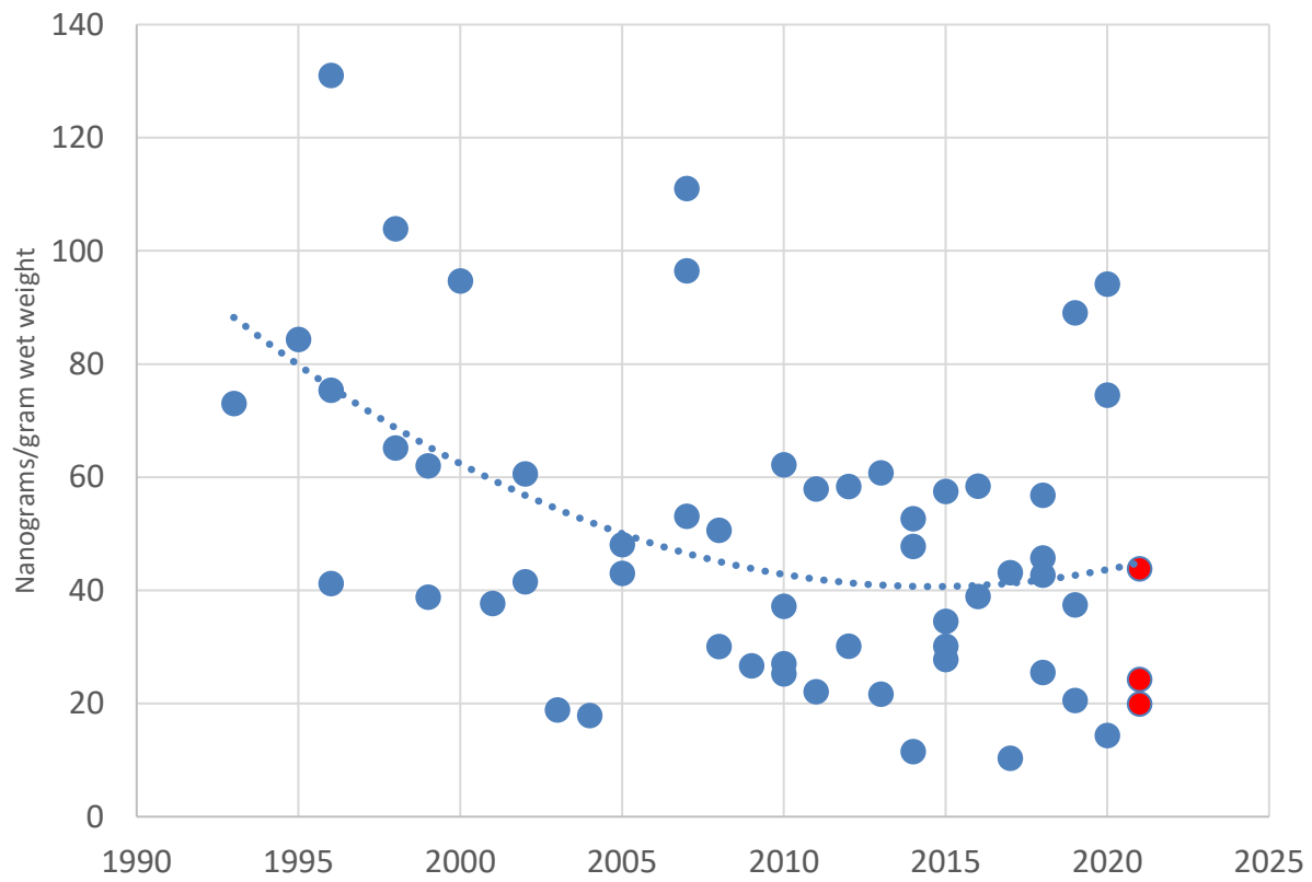
Total Chlordane
