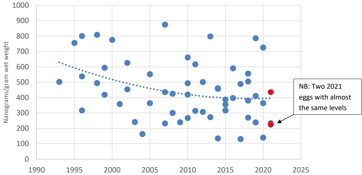
Total Chlordane
